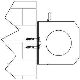
Wall Mounting
